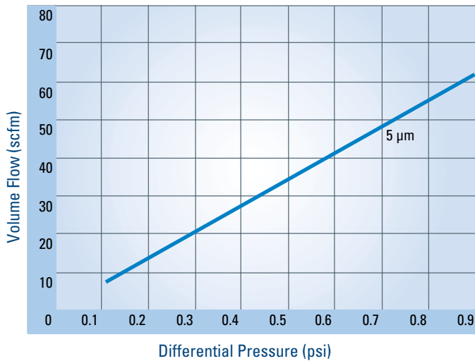
These curves define the flow of a 1030 filter element at standard conditions (14.7 psia; 68°F. R.H.= 70%)
