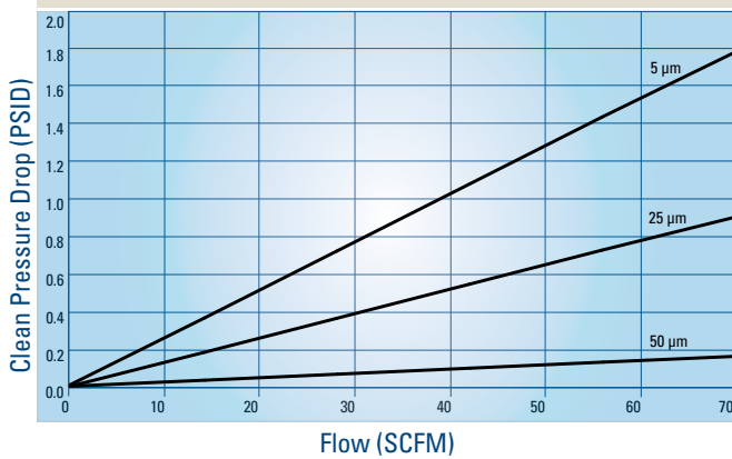
SBP Element Performance – Compressed Air
